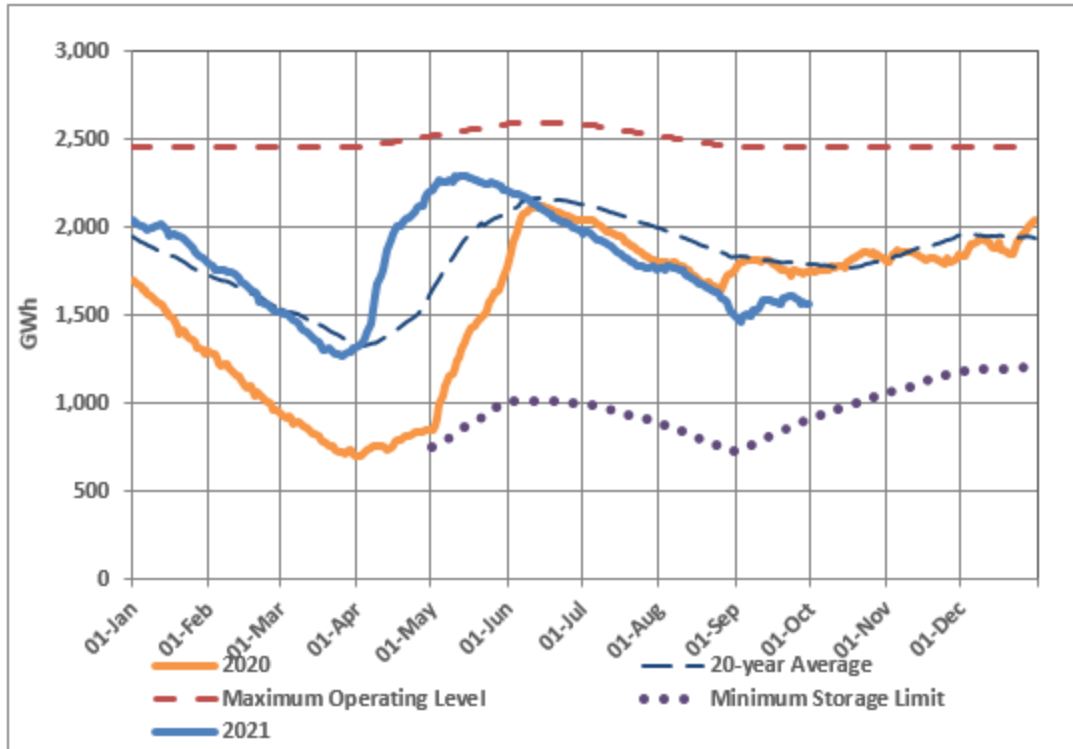
Figure 1: Total System Energy Storage for September 30, 2021
